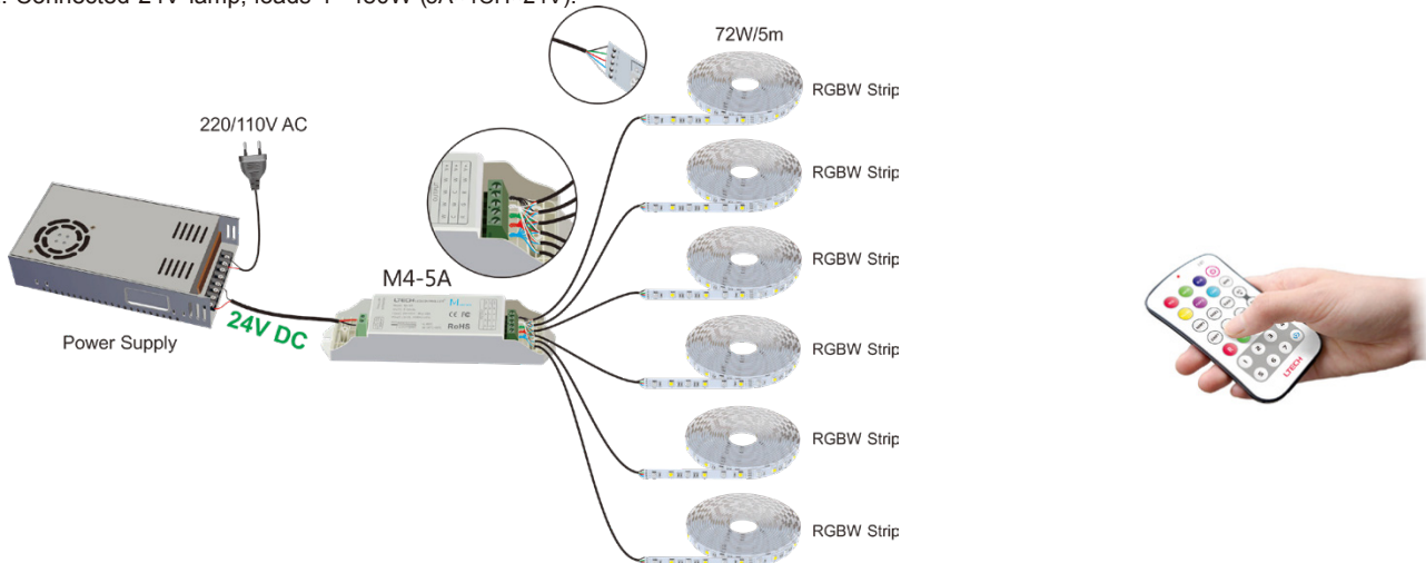
E.g. 2: Connected 24V lamp, loads 1~480W (5A×4CH×24V).
