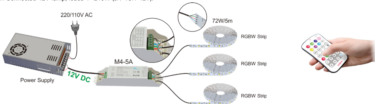
E.g. 1: Connected 12V lamp, loads 1~240W (5A×4CH×12V).
