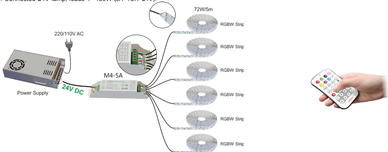
E.g. 2: Connected 24V lamp, loads 1~480W (5A×4CH×24V).
